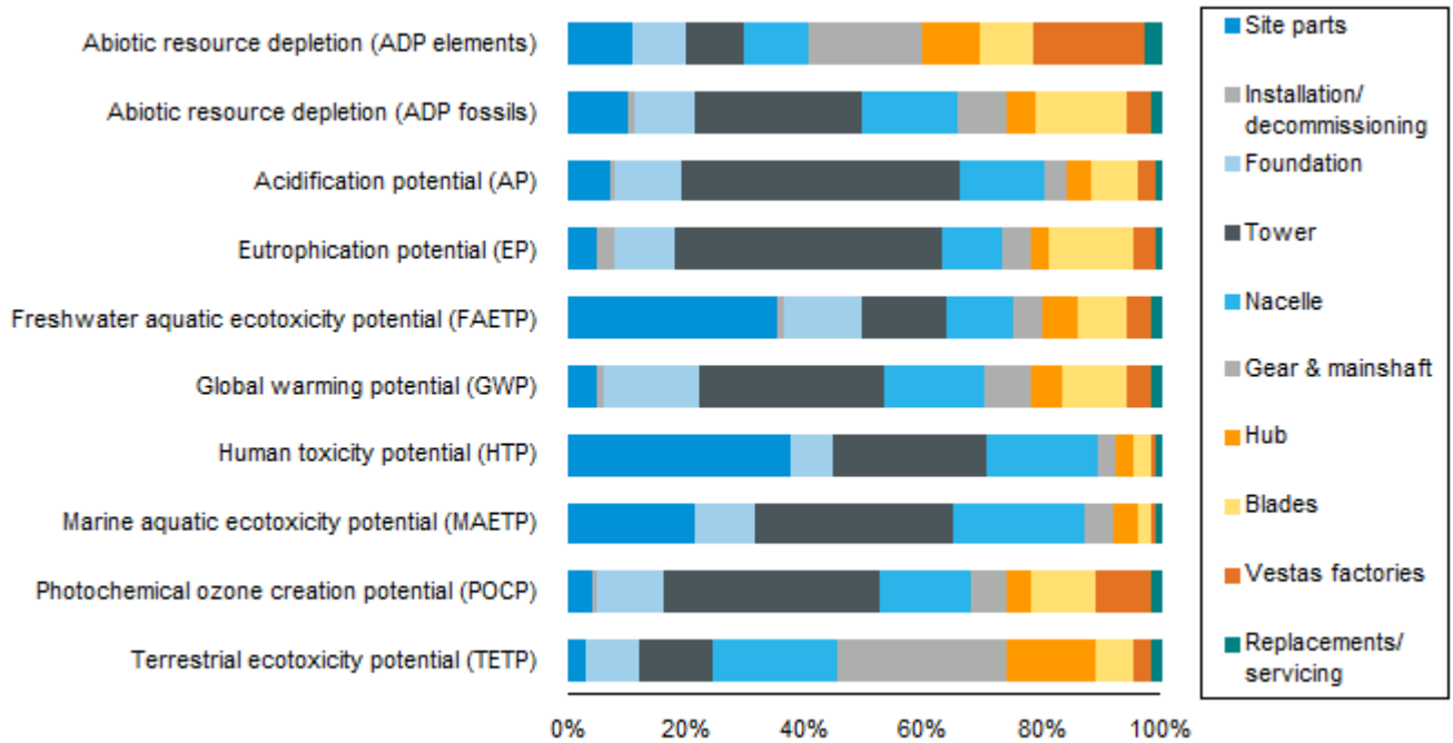
Figure 7: Production and use-phase environmental impacts of V117-3.45 MW
