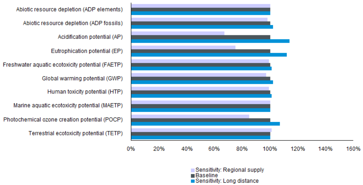
Figure 23: Whole-life sensitivity analysis of increased transport
