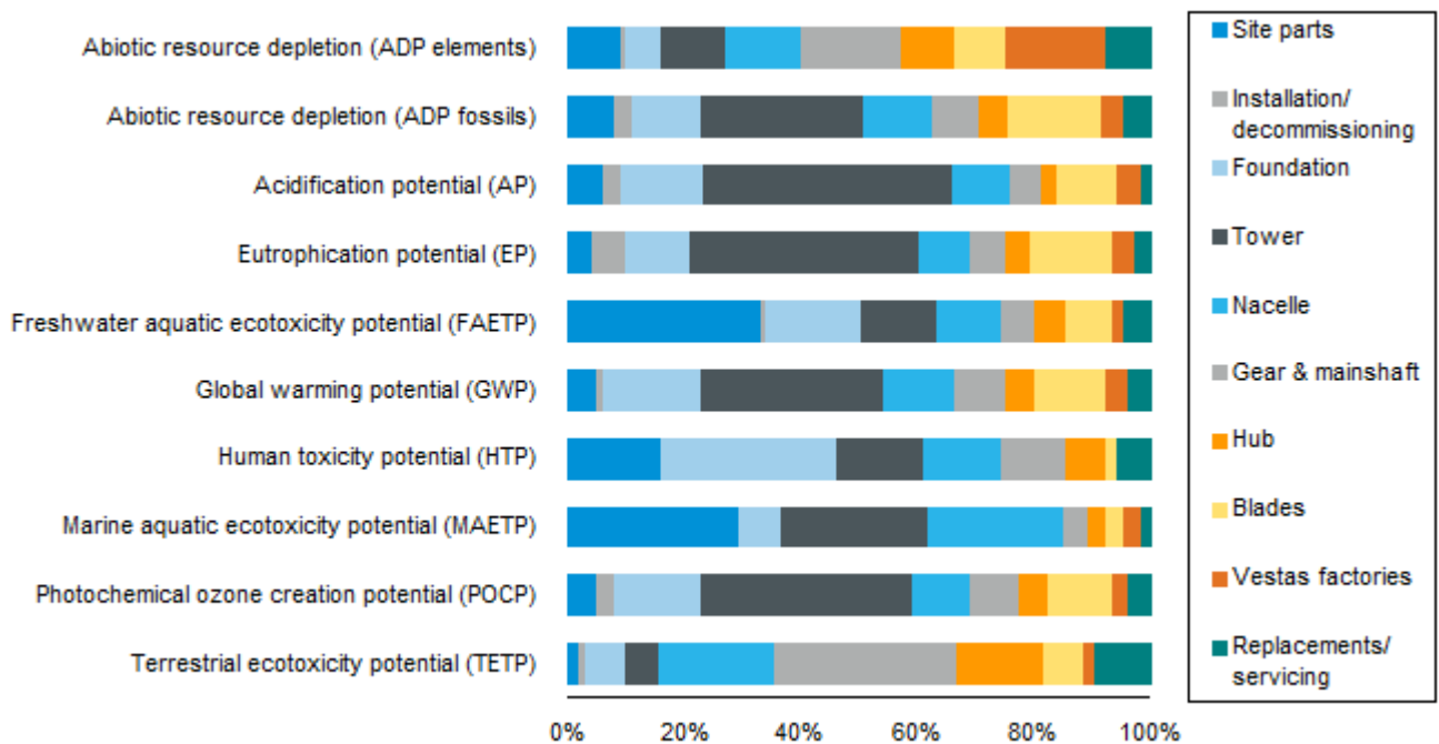
Figure 7: Production and use-phase environmental impacts of V117-4.2 MW
