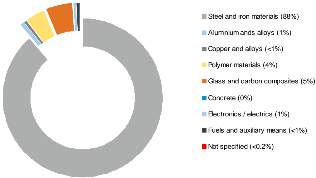
Figure 6: Material breakdown of 100MW power plant of V126-3.3 MW turbines (% mass)
