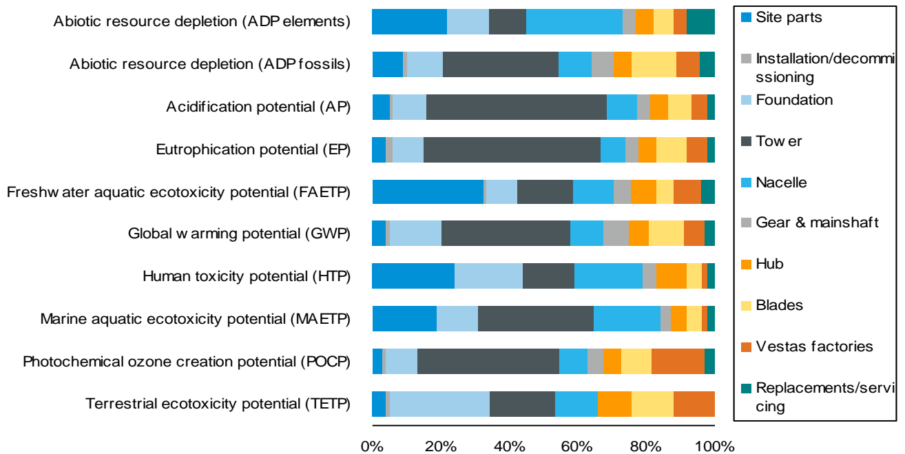
Figure 7: Production and use-phase environmental impacts of V126-3.3 MW
