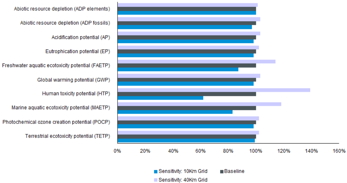
Figure 23: Whole-life impacts for doubling (40km) and halving (10km) distance to grid
