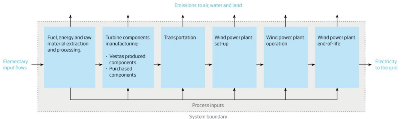
Figure 2: Scope of LCA for a 50MW onshore wind power plant of V110-2.0 MW turbines
