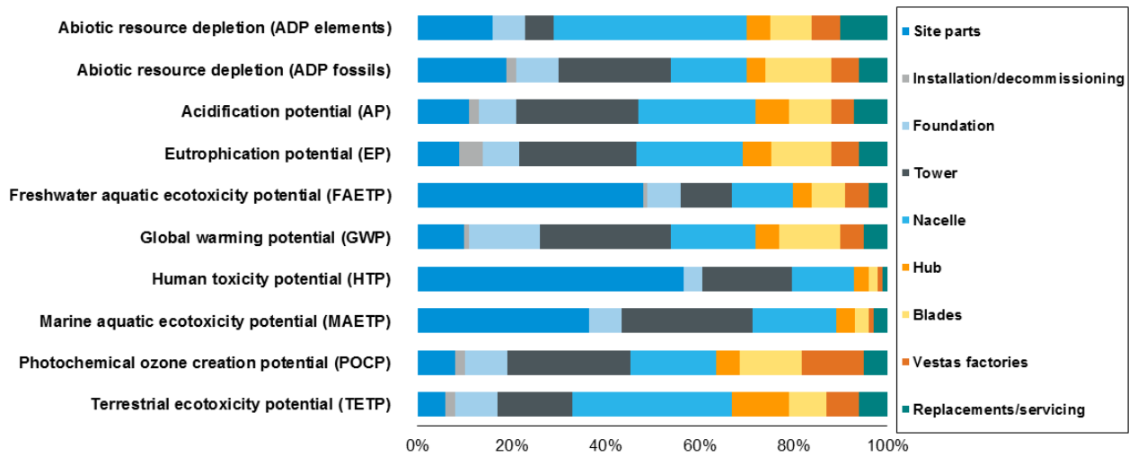
Figure 7: Production and use-phase environmental impacts of V110-2.0 MW
