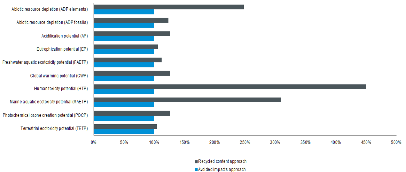
Figure 25: Whole-life impacts using a recycled-content approach for metal recycling credits
